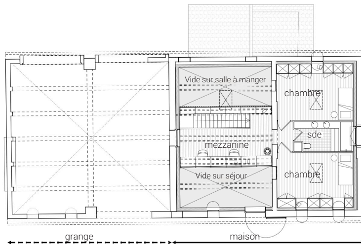
PLAN R+1
